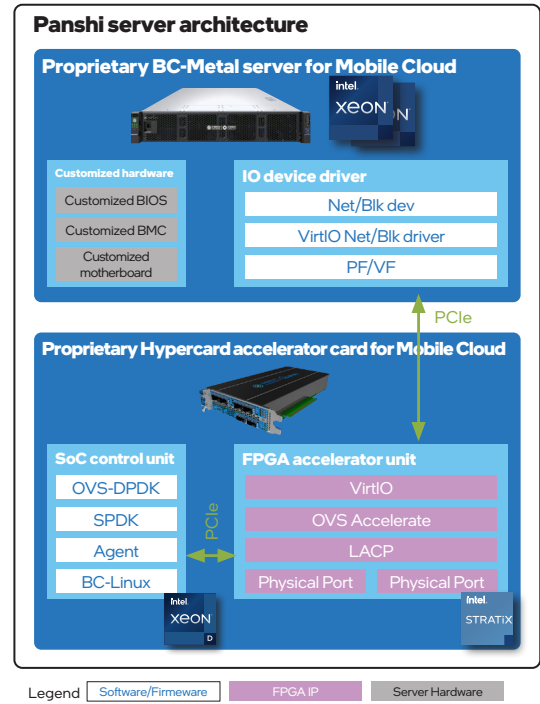
Figure 1. Mobile Cloud Panshi Server Architecture
