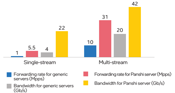
Figure 4. Comparative testing in network performance for the Panshi server architecture
