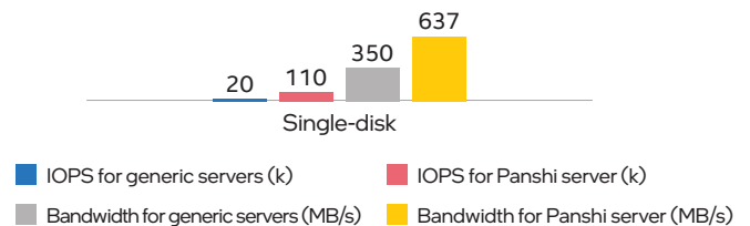
Figure 5. Comparative testing in storage performance for the Panshi server architecture
